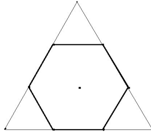
Figure 2: punctured hexagon
