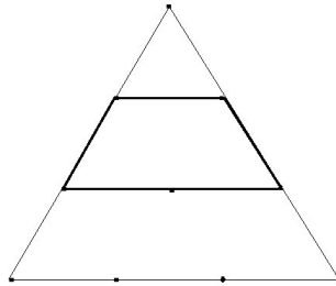
Figure 3: full trapezoid
