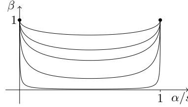
FIGURE 3. Optimal profiles (\alpha/s, \beta) obtained numerically from the minimization in the definition of g(s) , see (1.6), for f(z) = z/(1-z) and for s = 0.1, 0.3, 0.5, 1 , and 1.5 (from top to bottom). All curves remain inside the square (0, 1) \times (0, 1) except for the two endpoints.
