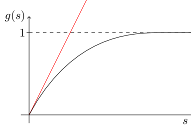
FIGURE 2. Sketch of the function g(s) defined in (1.6), obtained by numerical minimization using f(z) = z/(1-z) (cp. Proposition 4.1 and Remark 4.2).
