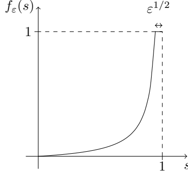
FIGURE 1. Sketch of the function f_\varepsilon(z) for the prototypical case f(z) = z/(1-z) .
