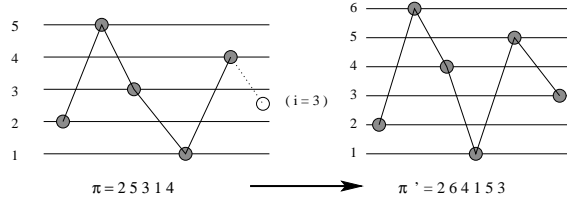
Figure 1: an ECO construction for permutations by adding a new node in the rightmost position
