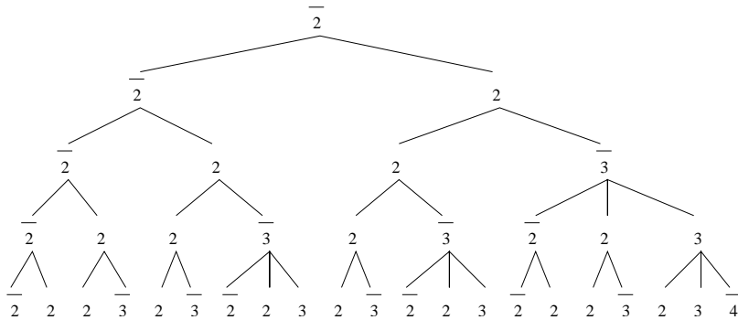
Figure 5: the generating tree of S(1 - 23, 21 - 3)
