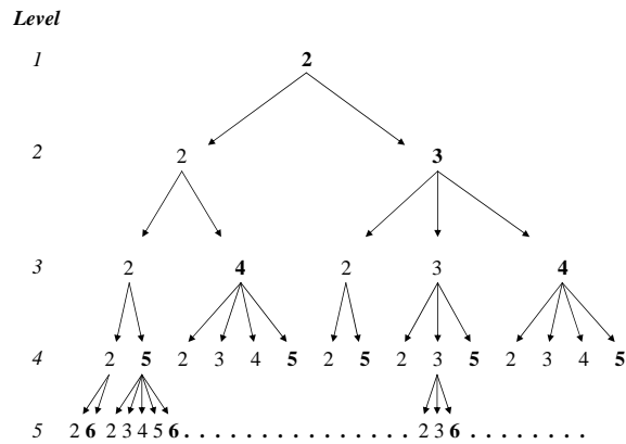
Figure 3: the generating tree of \Omega
